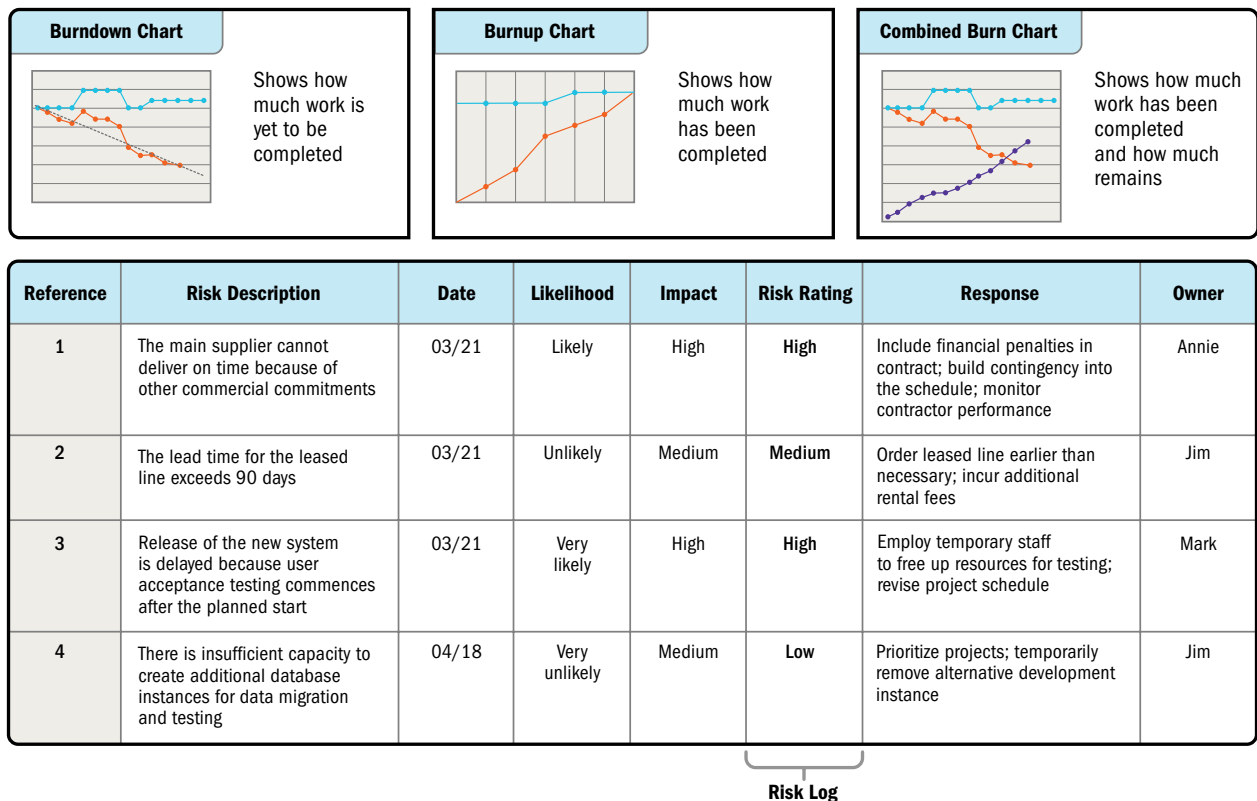
Figure 2-28. Information Radiator
